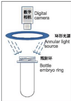
Optical path design
